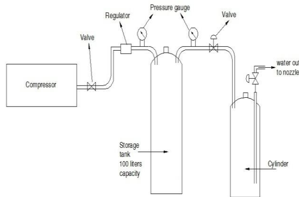
Fig. 6: Opposed jet spray generation system
