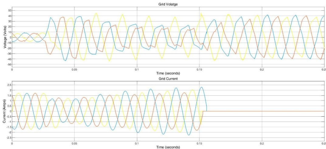
Figure 4 Grid Voltages and Current
