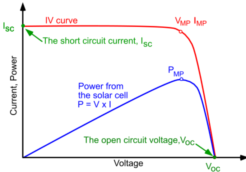
Figure 3 PV Panel Characteristic Curves [18]
