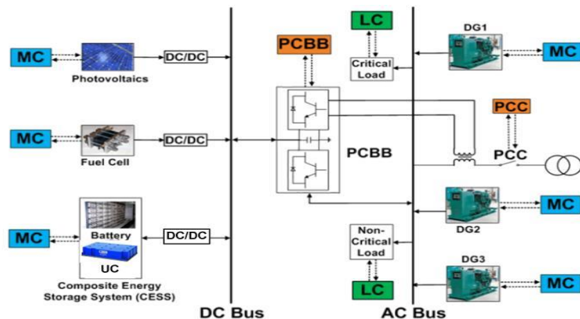
Figure 2 Architecture Diagram
