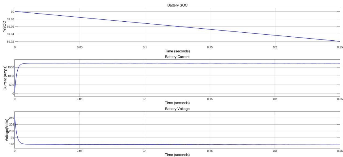
Figure 5 Battery Output
