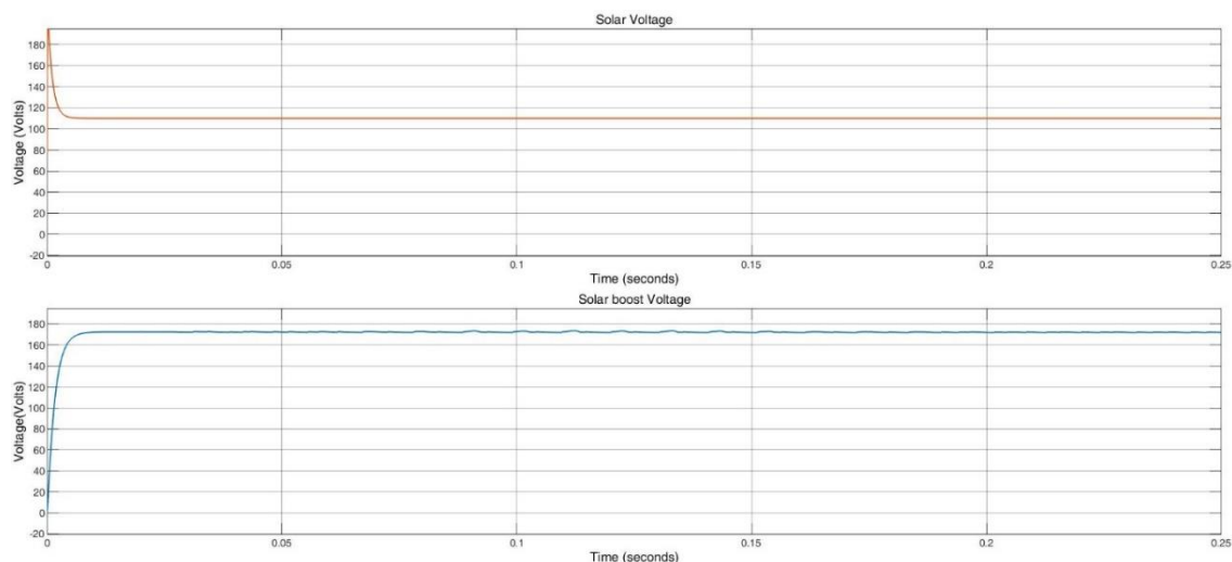
Figure 6 Solar Voltages: Before and after boost converter
