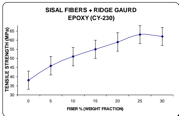
Fig: 2 Tensile Strength of Epoxy-Sisal-Ridge Gourd-Hybrid-Composite.
