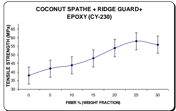
Fig: 3 Tensile Strength of Epoxy-Coconut Spathe-Ridge Gourd-Hybrid-Composite.
