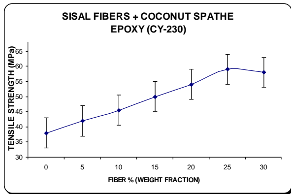
Fig: 1 Tensile Strength of Epoxy-Sisal-Coconut spathe-Hybrid-Composite.
