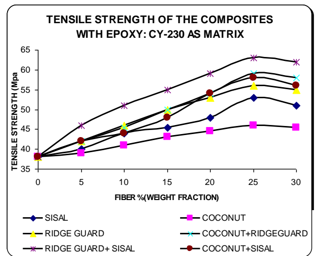
Fig: 4 Tensile strengths of the composites with EPOXY-CY-230 as Matrix.
