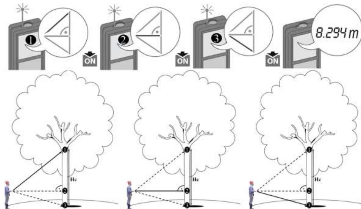
Fig. 1. Procedure for obtaining commercial height. The distances 1, 2 and 3 are measured as indicated on the display. After measurement 3, the commercial height of the tree, in meters, is displayed on the device screen
