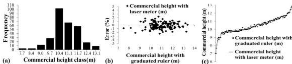
Fig. 2. Frequency distribution of trees with commercial height greater than 7 m and less than 14 m (a), distribution of residuals of height, in percentage, for the laser meter method (b) and line estimate of the heights measured with laser meter (c)
