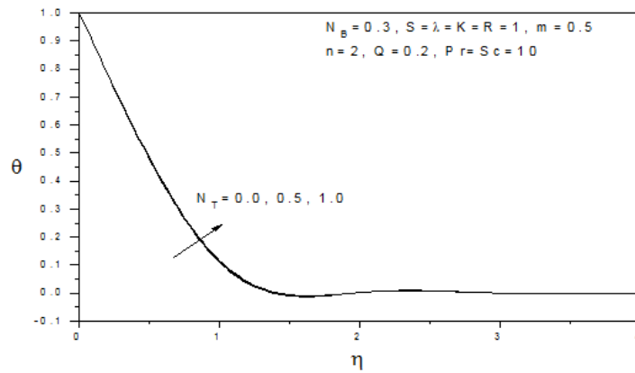
Fig.1(c) Temperature profiles for different values of N_T
