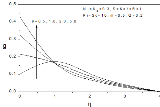
Fig.3 (b) Angular velocity profiles for different values of n
