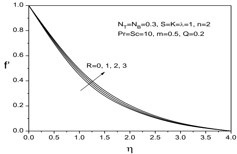
Fig.10(a) Velocity profiles for different values of R
