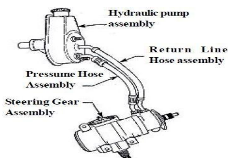
Figure 6: Power Steering Gear
