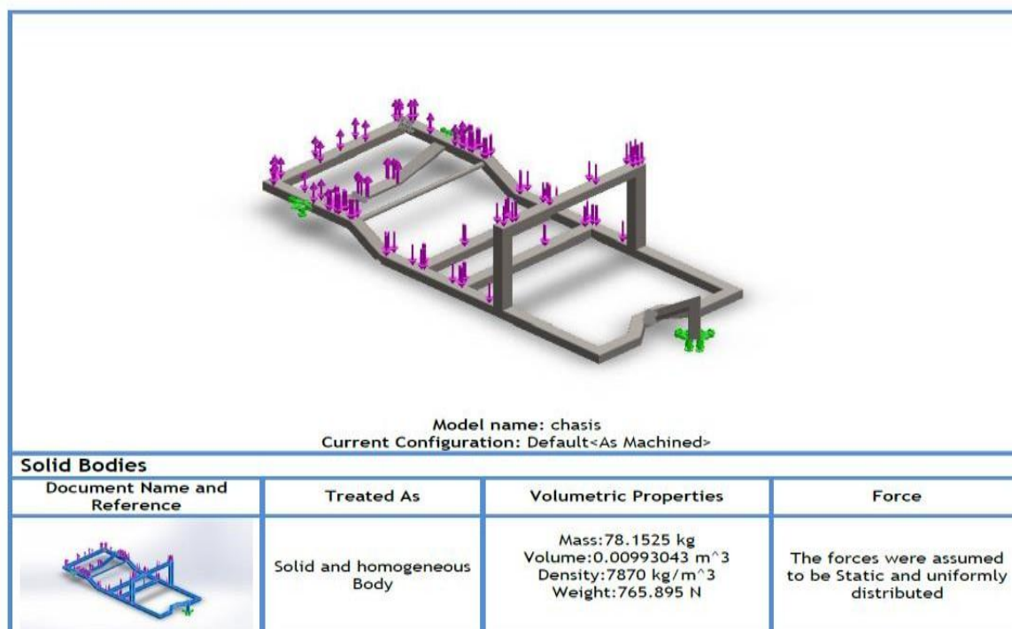
Figure 1: The model information of the chassis
