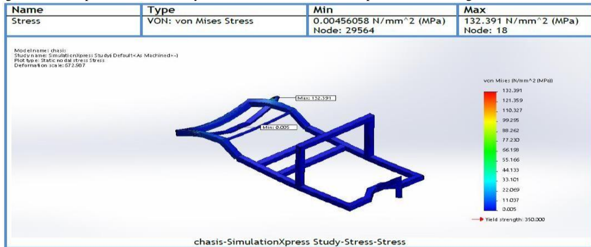
Figure 3: Chassis frame maximum and minimum stresses
