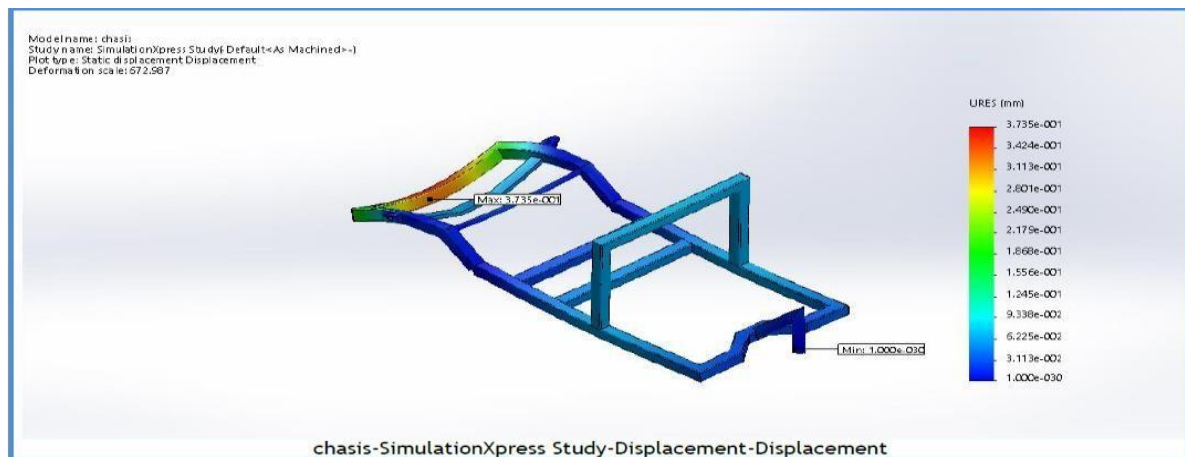
Figure 4: Chassis frame static displacement
